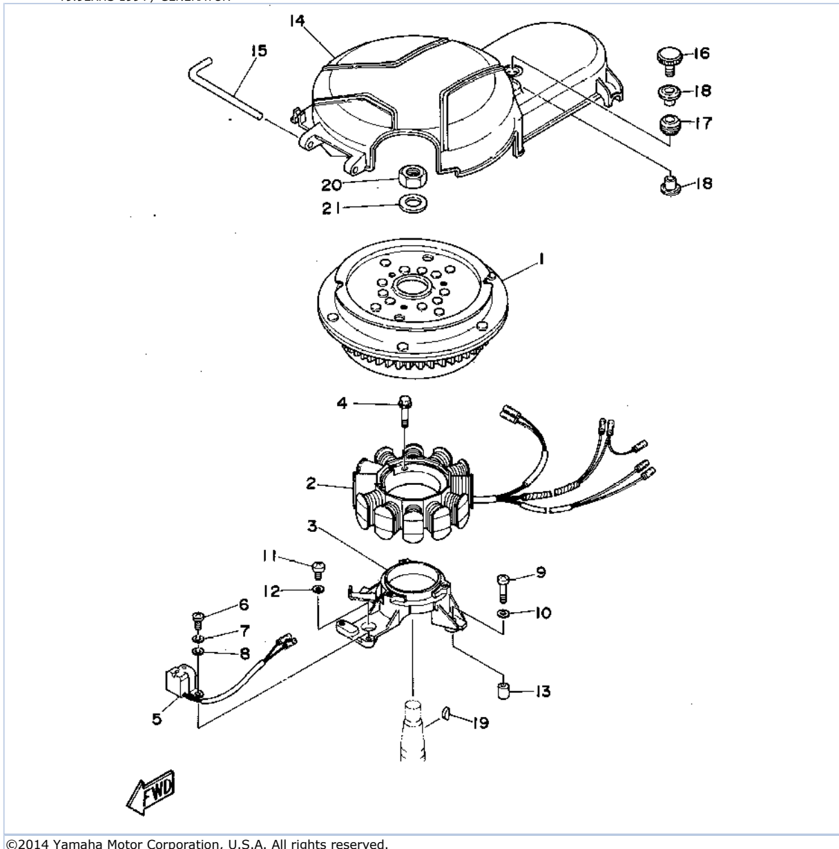
T9.9EXHS 1994 / GENERATOR
