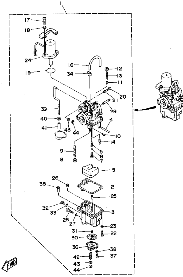
T9.9EXHS 1994 / CARBURETOR
