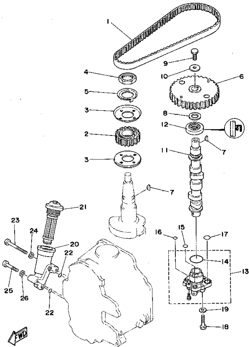
T9.9EXHS 1994 / OIL PUMP
