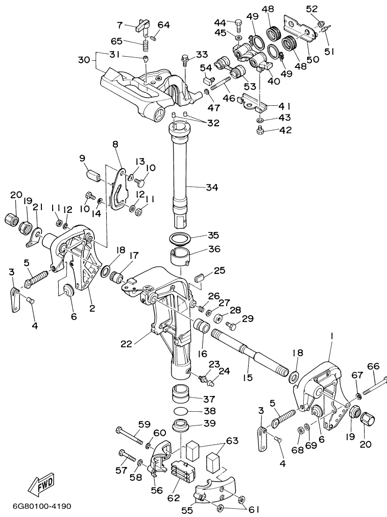
T9.9ELHD 2005 / BRACKET 1
