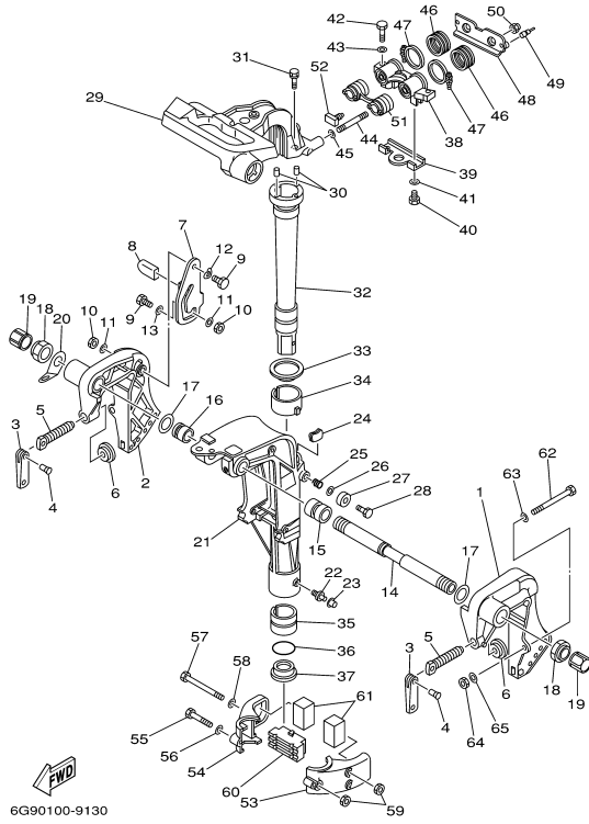
F9.9ELRX 1999 / BRACKET 1
