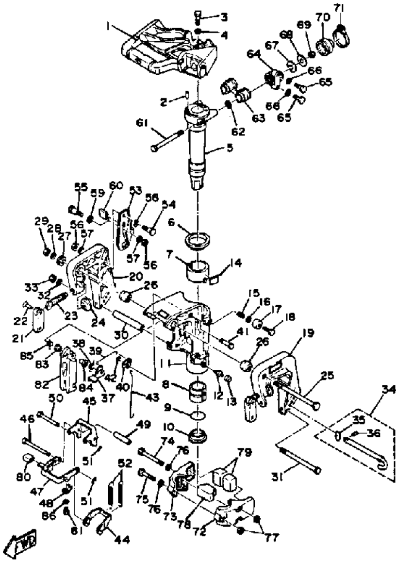
9.9ELJ 1986 / BRACKET
