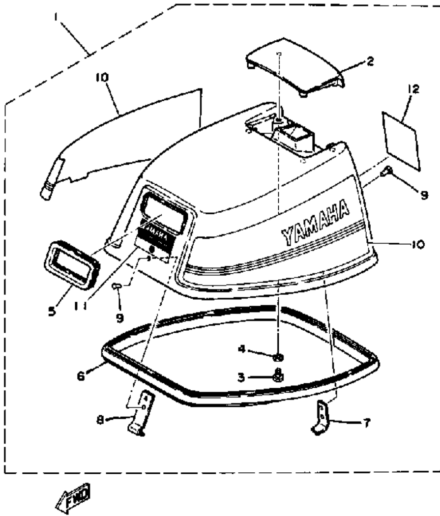
6SJ 1986 / TOP COWLING 6H 8H
