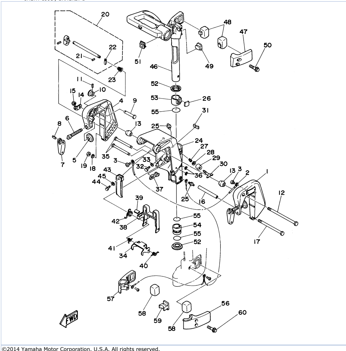
6MSHT 1995 / BRACKET 1
