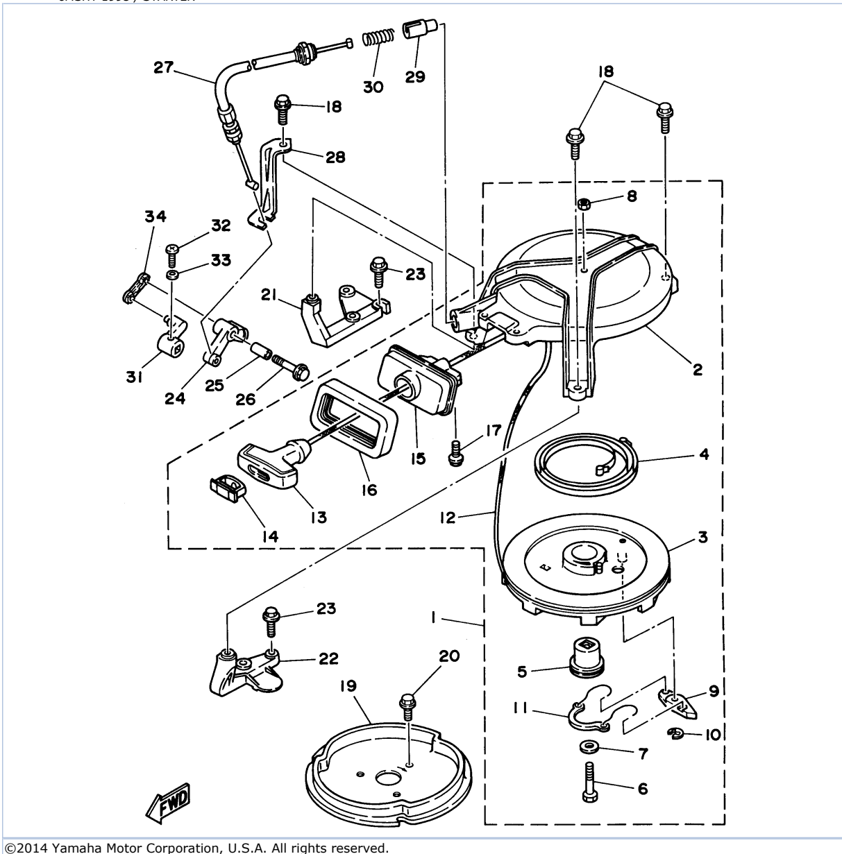
6MSHT 1995 / STARTER
