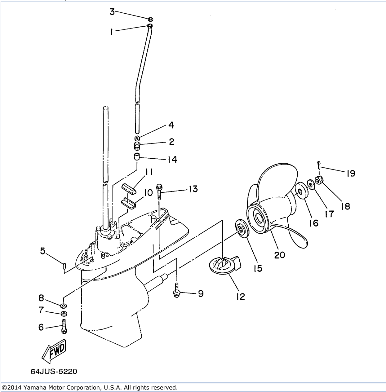
T50TLRX 1999 / LOWER CASING DRIVE 2 T50TLRX
