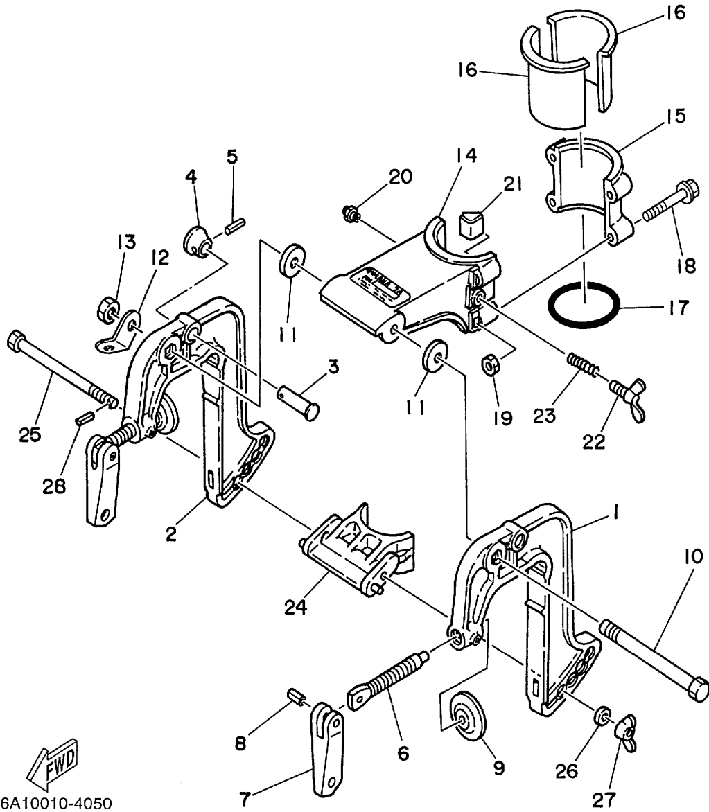
2MSHX 1999 / BRACKET 1
