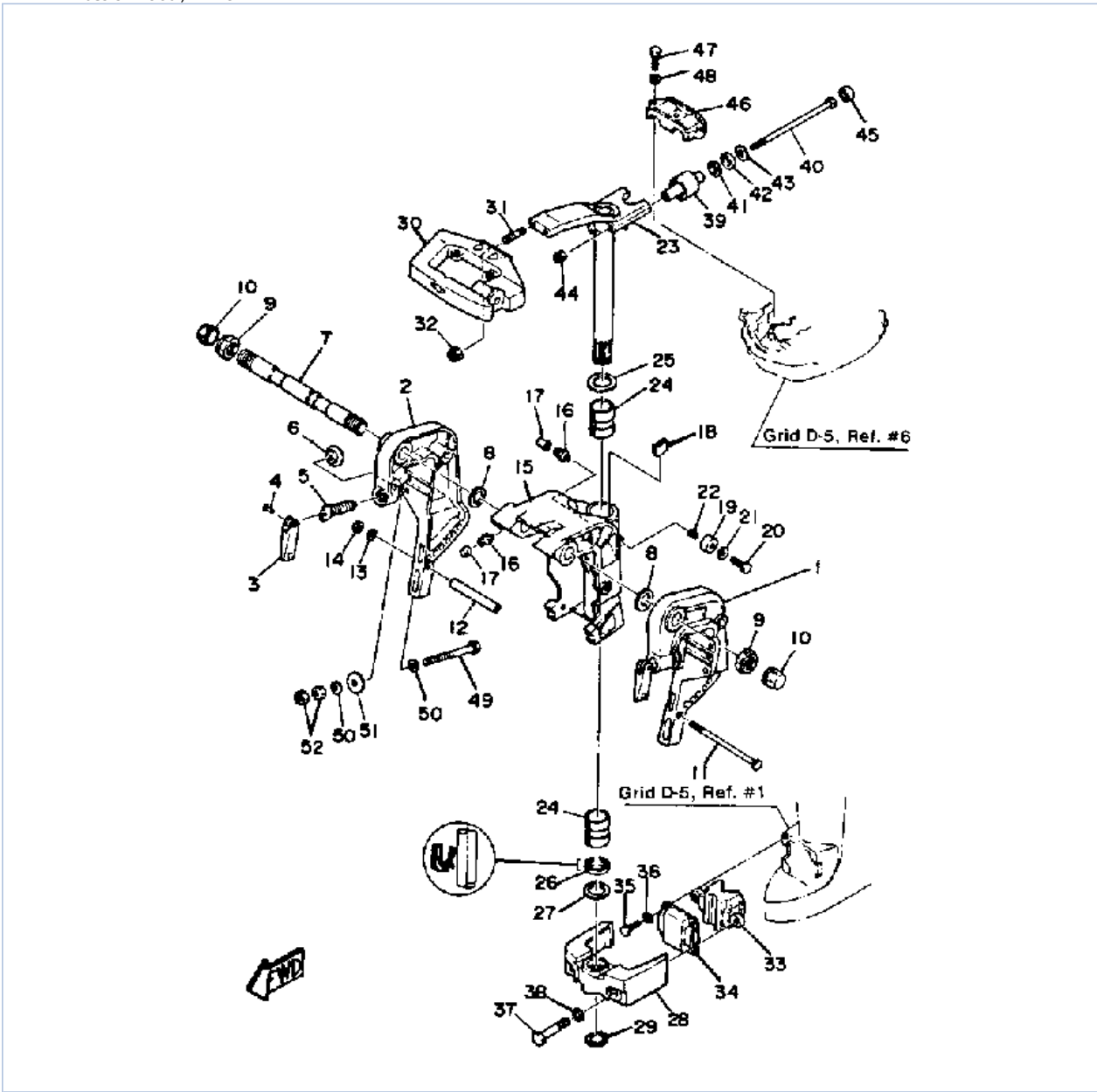
40SJ-JD 1986 / BRACKET 1
