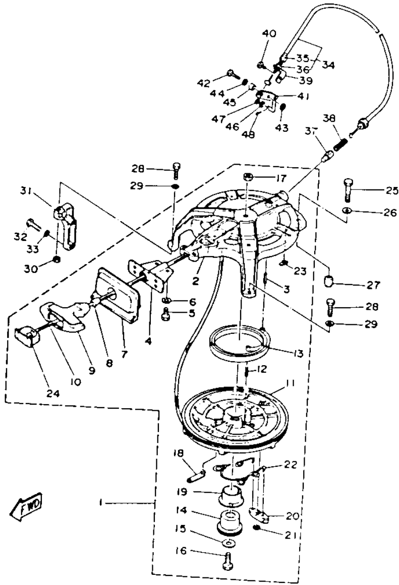
C25ELRP 1991 / MANUAL STARTER
