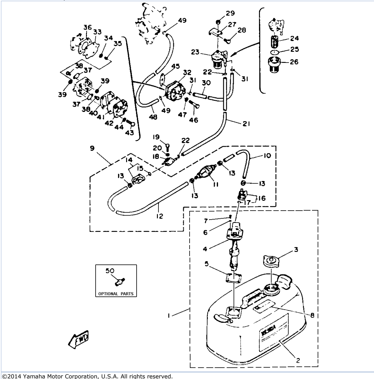
C25ELRP 1991 / FUEL TANK
