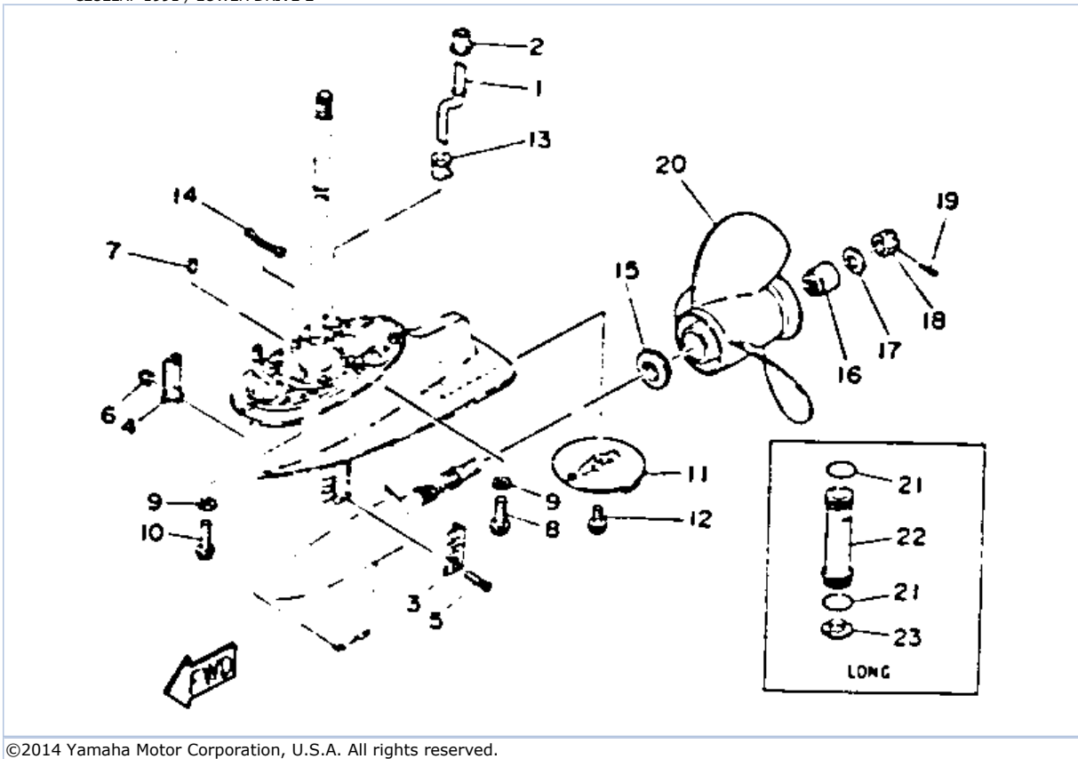
C25ELRP 1991 / LOWER DRIVE 2
