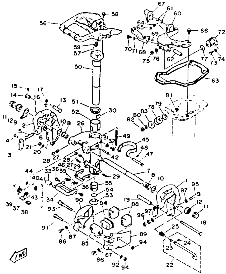
C25ELHP 1991 / BRACKET 1
