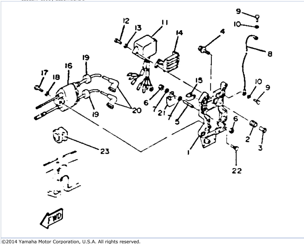
C25ELHP 1991 / ELECTRICAL 1
