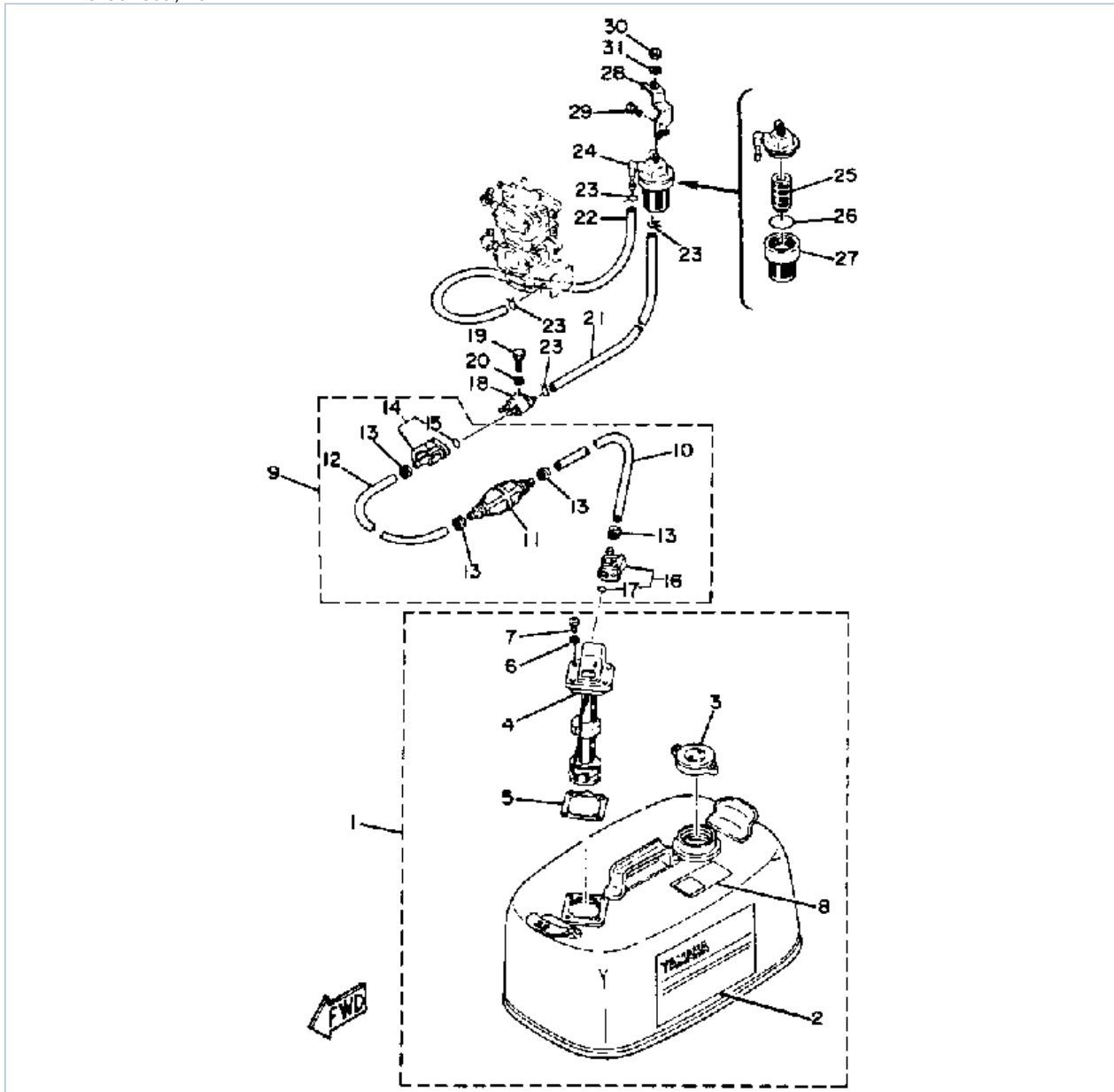
25ESG 1988 / FUEL TANK
