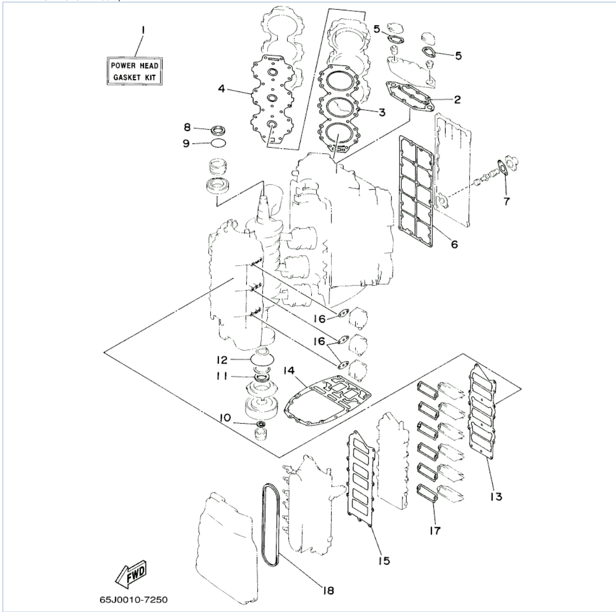
SX225TURA 2002 / REPAIR KIT 1
