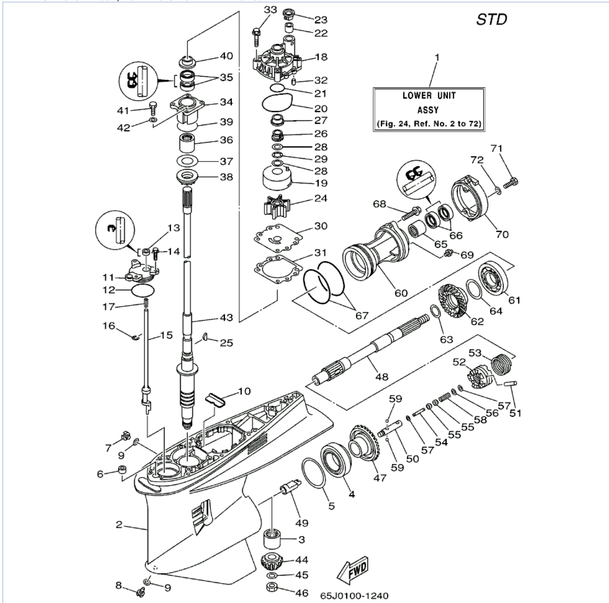
SX225TURA 2002 / LOWER CASING DRIVE 1 225 250
