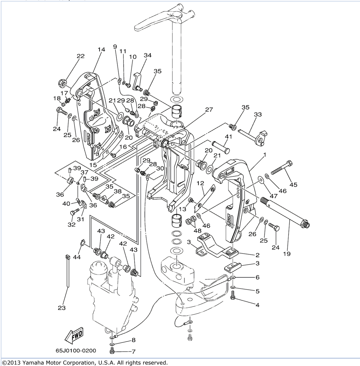
SX225TURA 2002 / BRACKET 1
