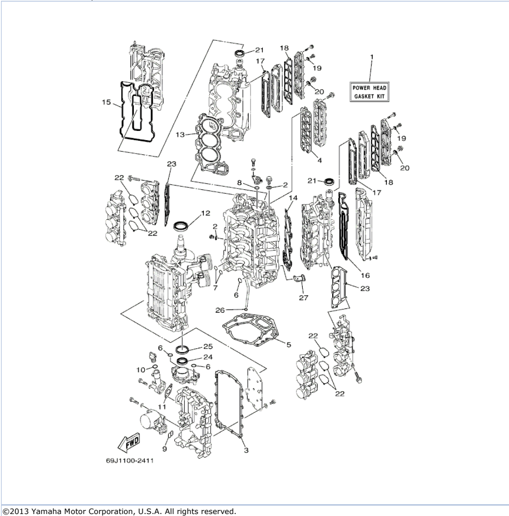
F225TURA 2002 / REPAIR KIT 1
