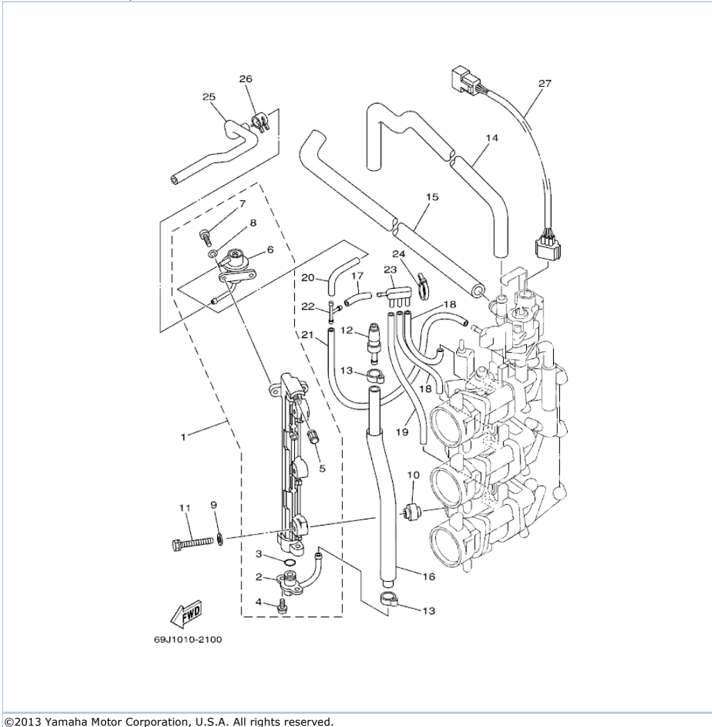
F225TURA 2002 / THROTTLE BODY ASSY 3
