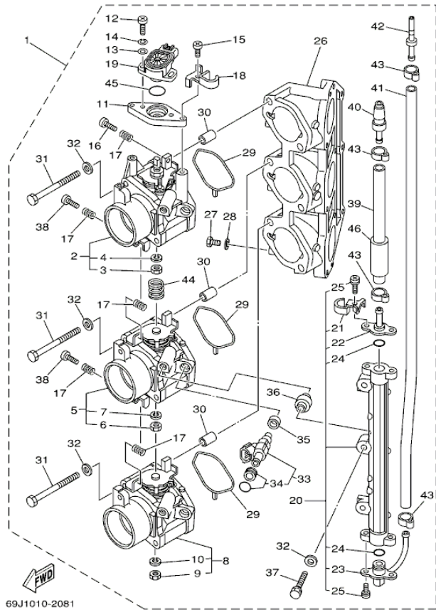
F225TURA 2002 / THROTTLE BODY ASSY 1
