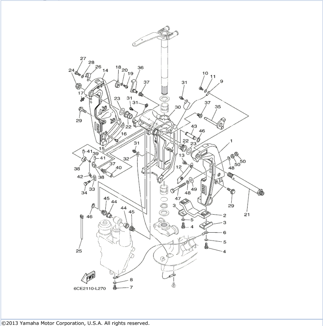
LF225XCA_0411 / BRACKET 1
