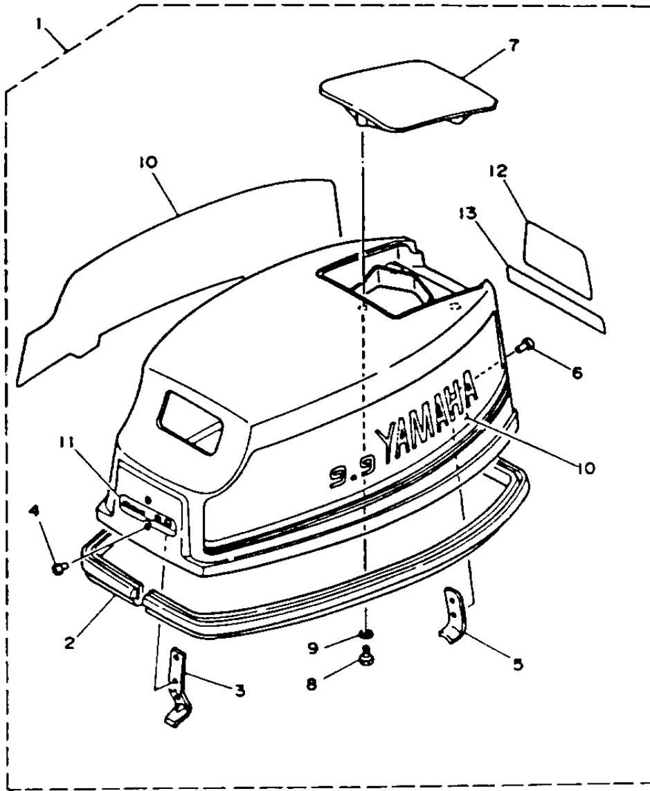
15ESHR 1993 / TOP COWLING
