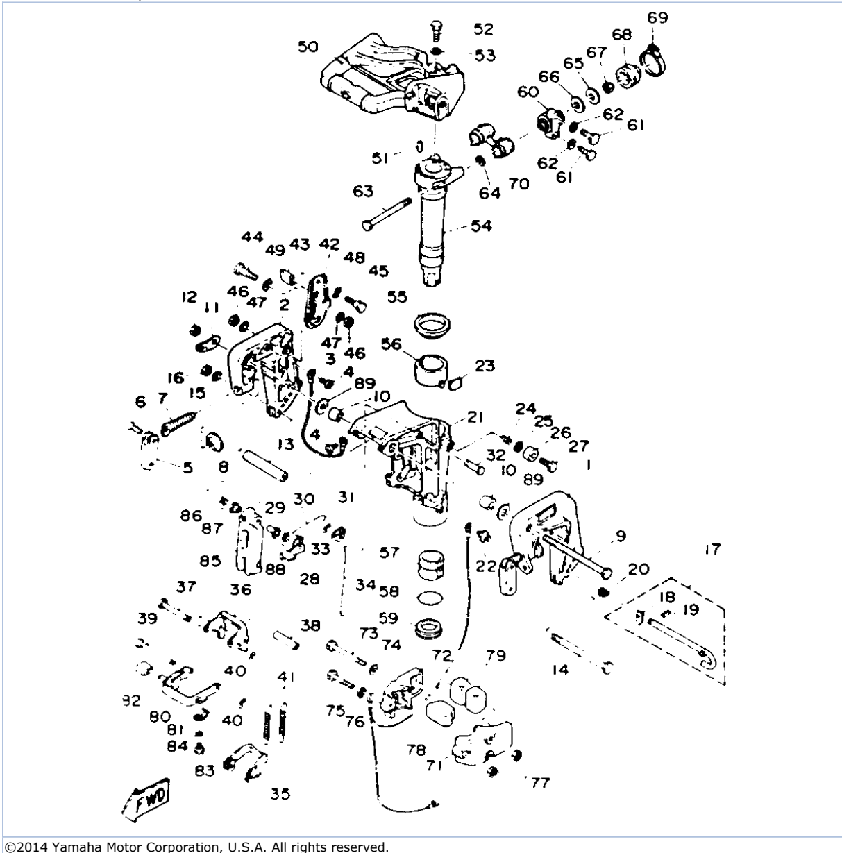
15ESHR 1993 / BRACKET
