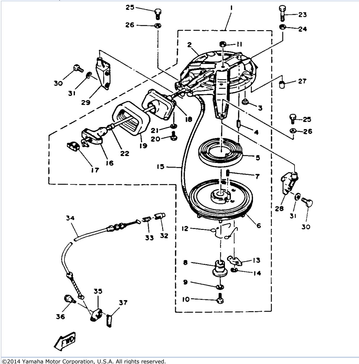
15ESHR 1993 / MANUAL STARTER
