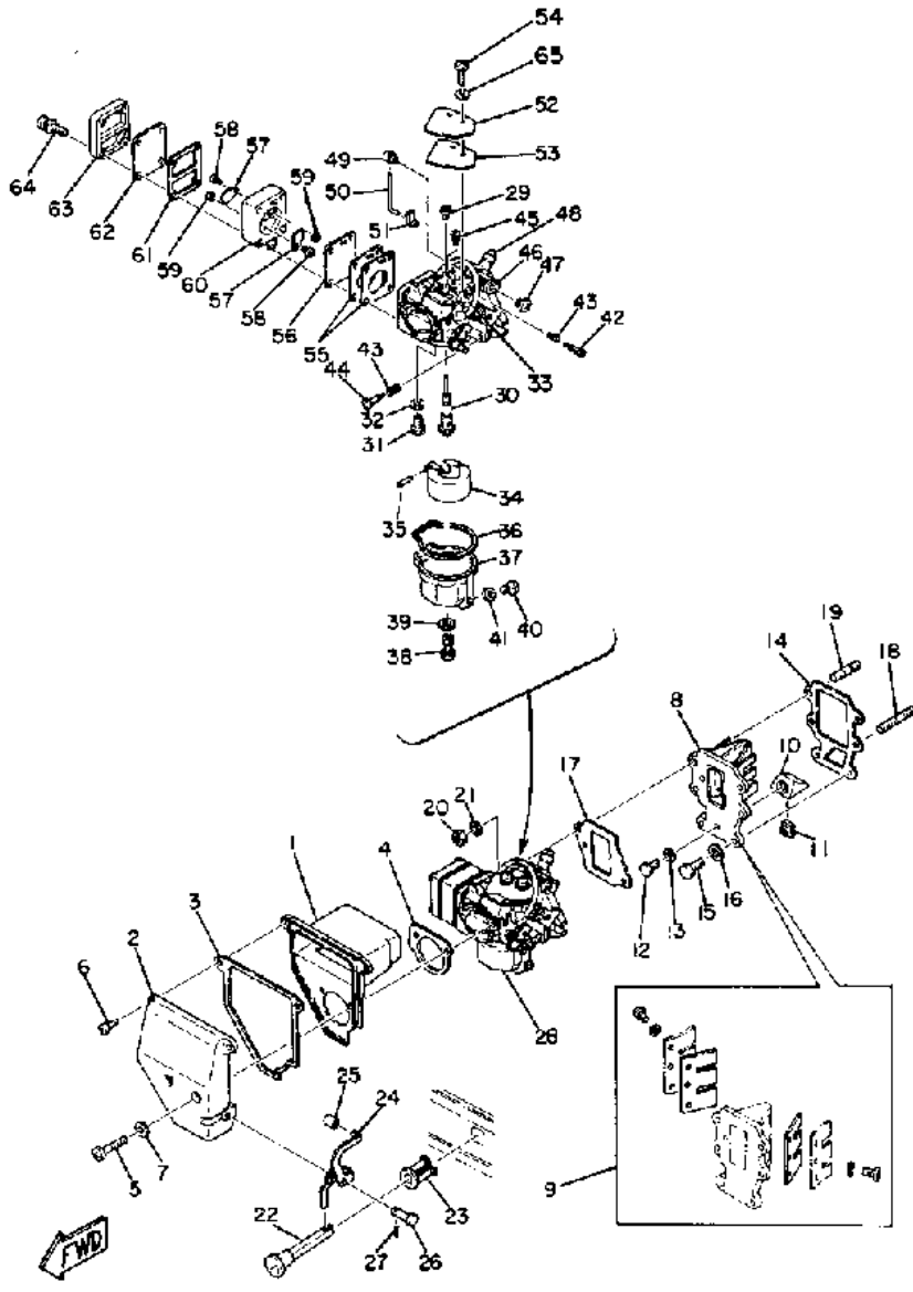
15ELJ 1986 / AIR CLEANER CARBURETOR (9.9H 15H)
