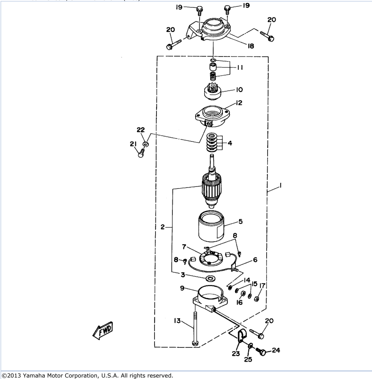
P200TLRS 1994 / STARTING MOTOR 2 (P200)
