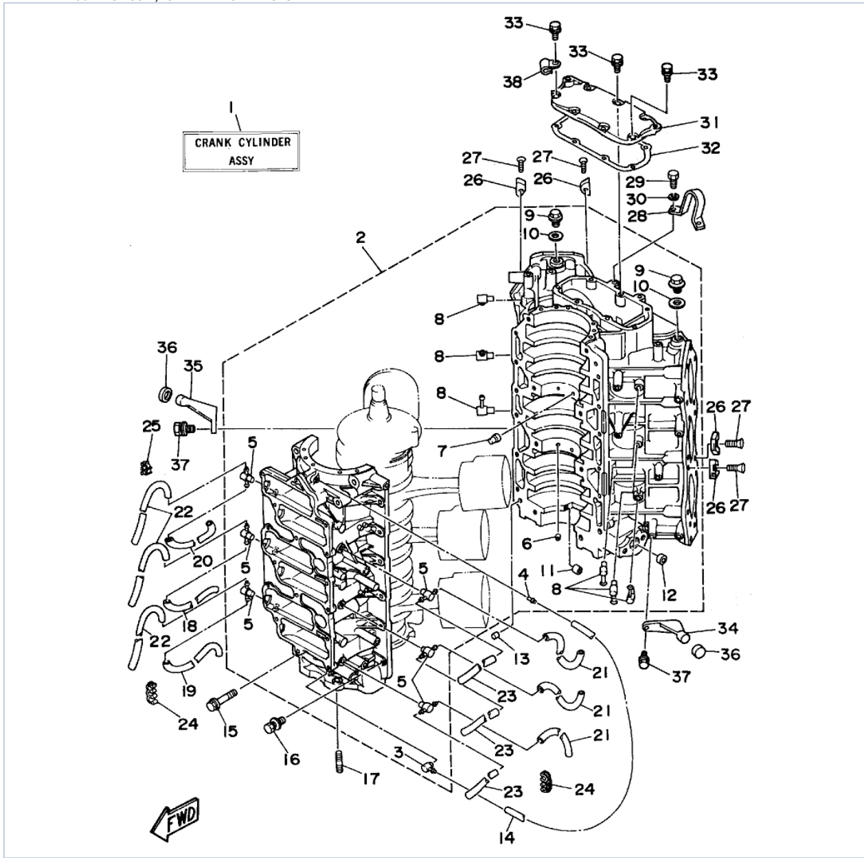
P200TLRS 1994 / CYLINDER CRANKCASE 1
