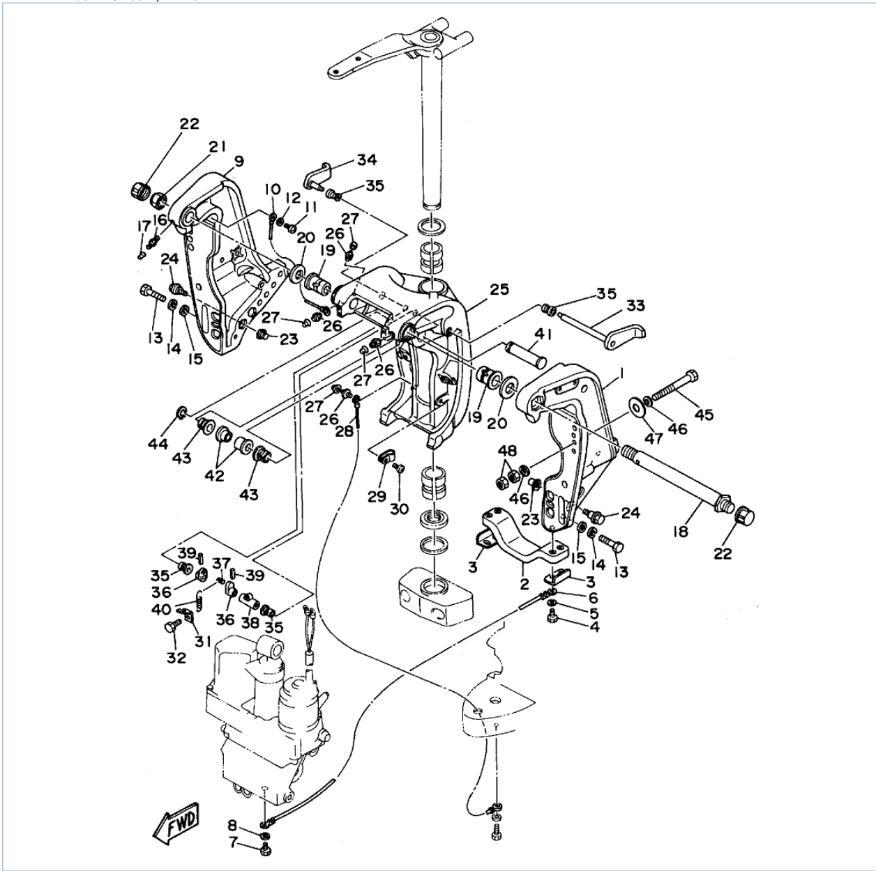
P200TLRS 1994 / BRACKET 1
