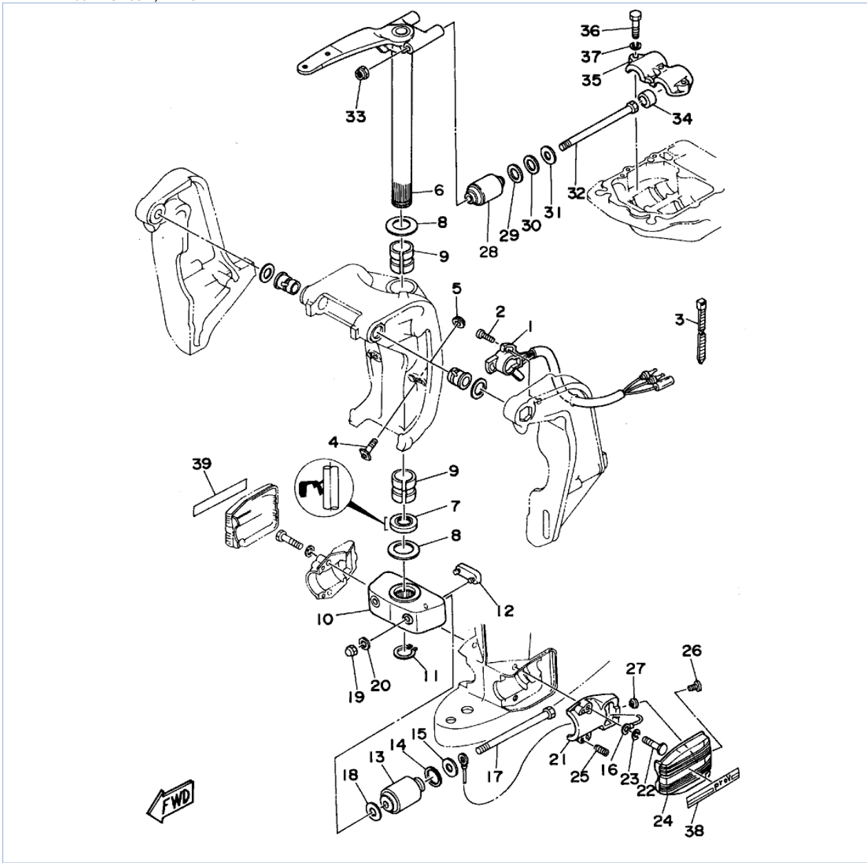
P200TLRS 1994 / BRACKET 2
