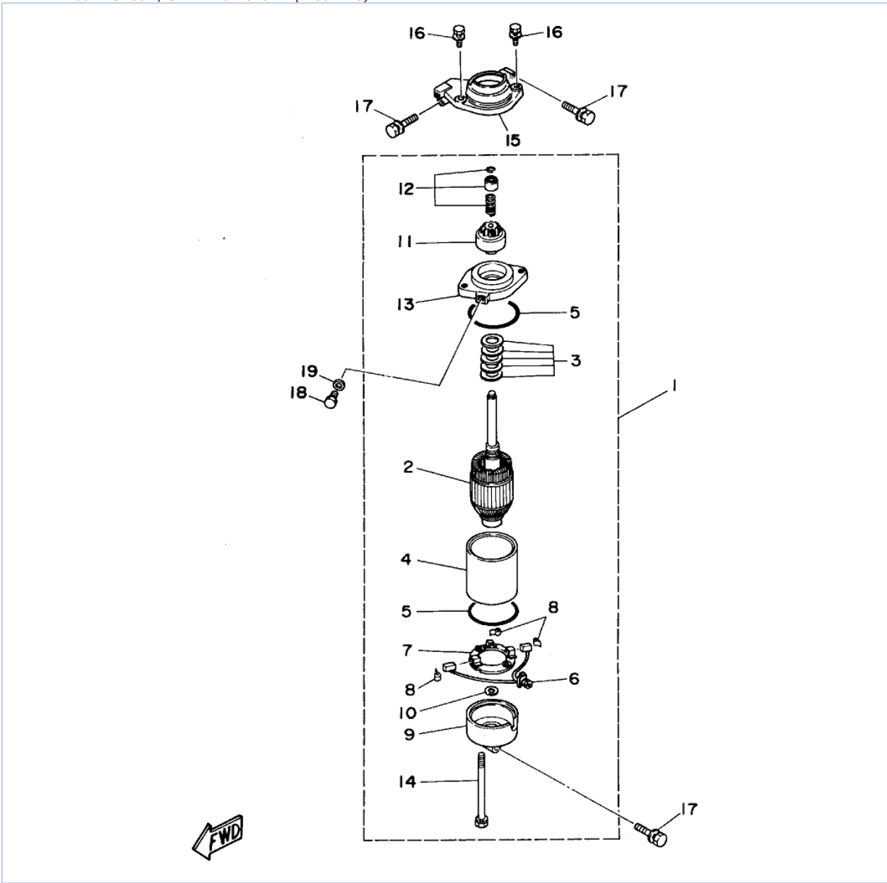
P200TLRS 1994 / STARTING MOTOR 1 (P150 P175)
