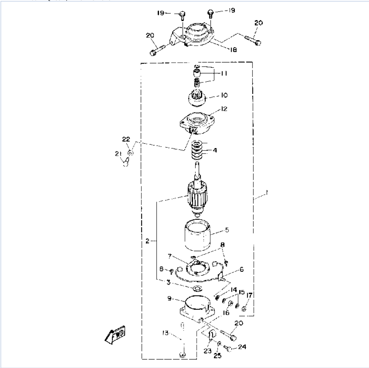
P200TLRQ 1992 / ELECTRIC MOTOR
