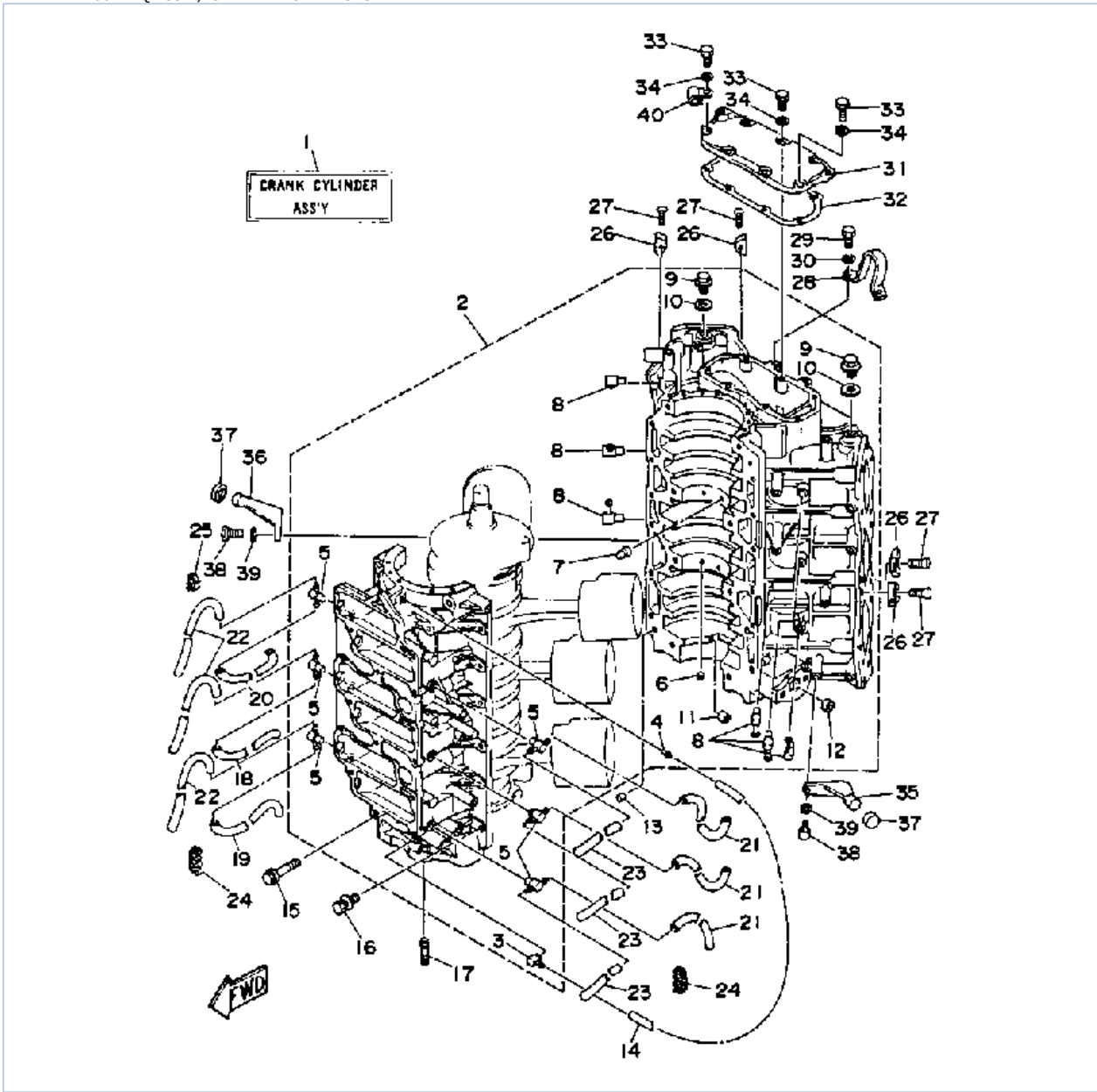
P200TLRQ 1992 / CYLINDER CRANKCASE 1
