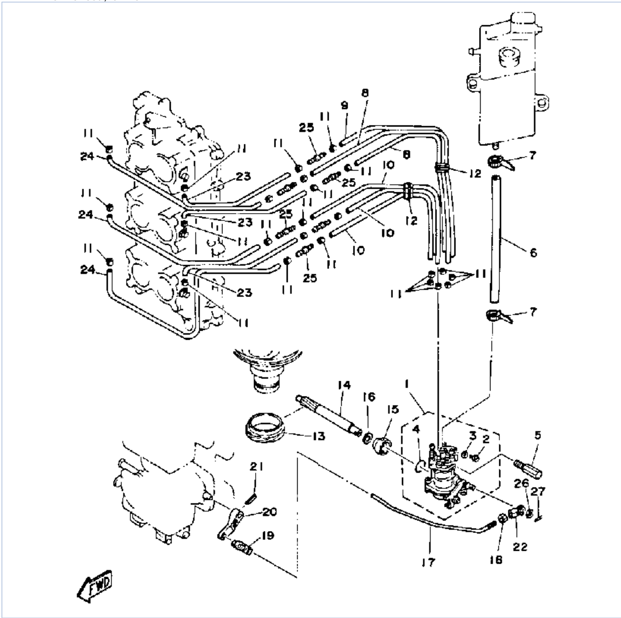
175ETXJ 1986 / OIL PUMP
