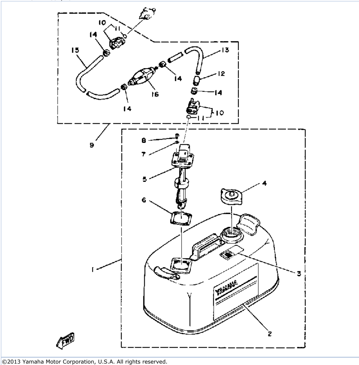
175ETLN 1984 / FUEL TANK
