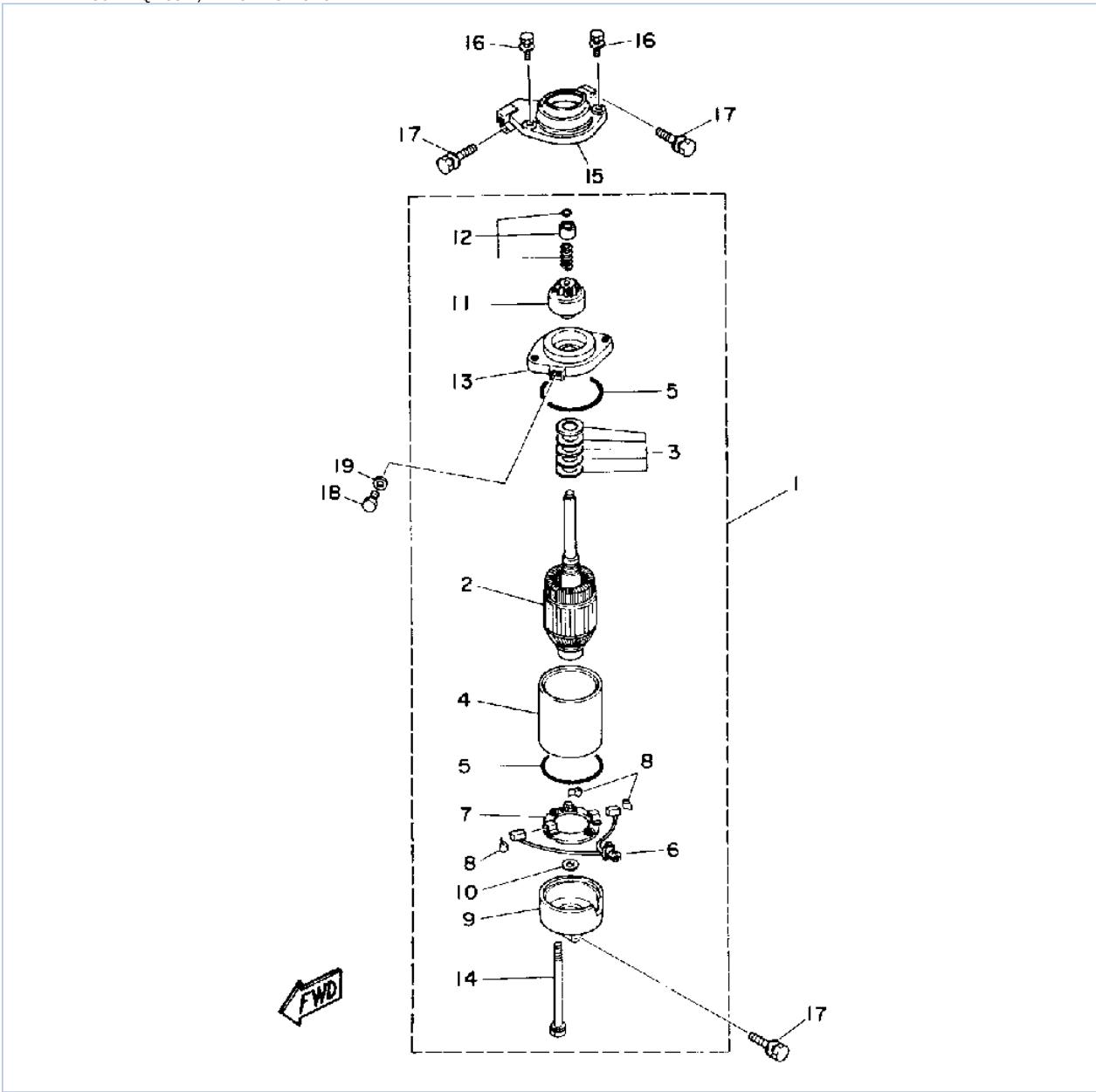
L150TXRQ 1992 / ELECTRIC MOTOR
