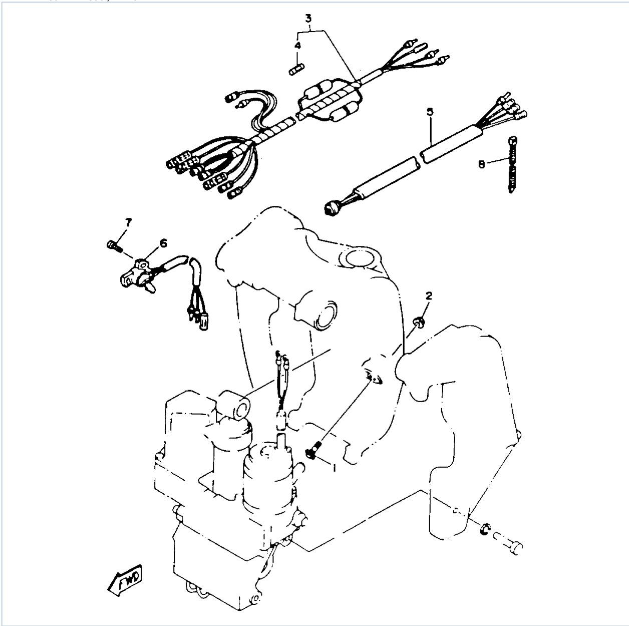
150TLRR 1993 / BRACKET 2
