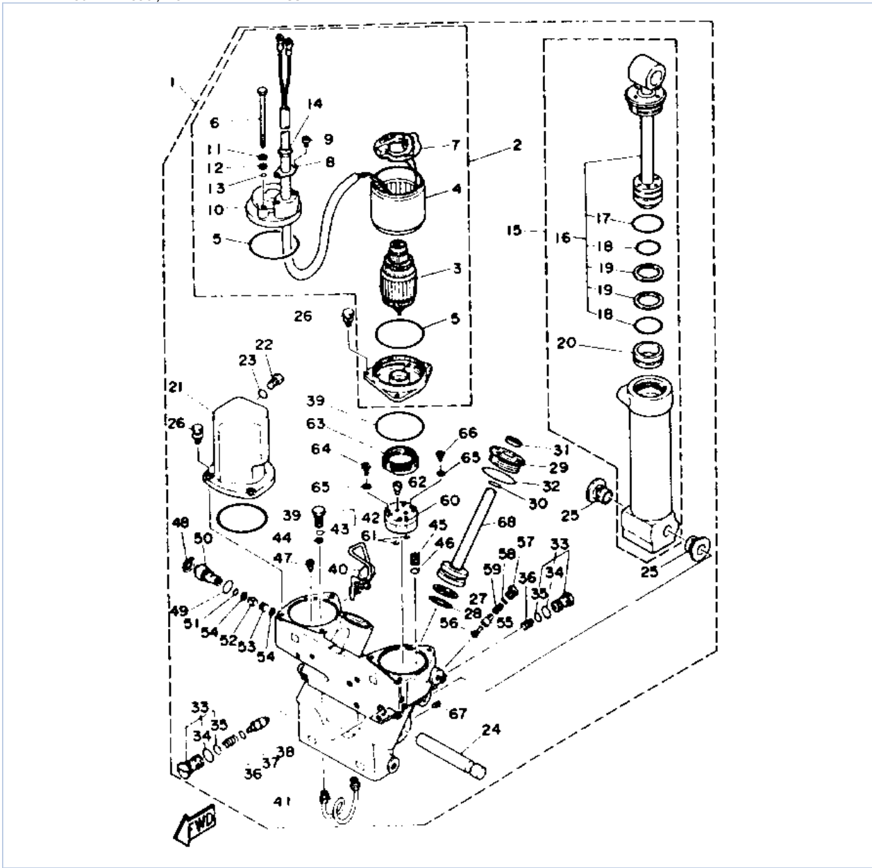
L150TXRR 1993 / POWER TRIM TILT ASSEMBLY
