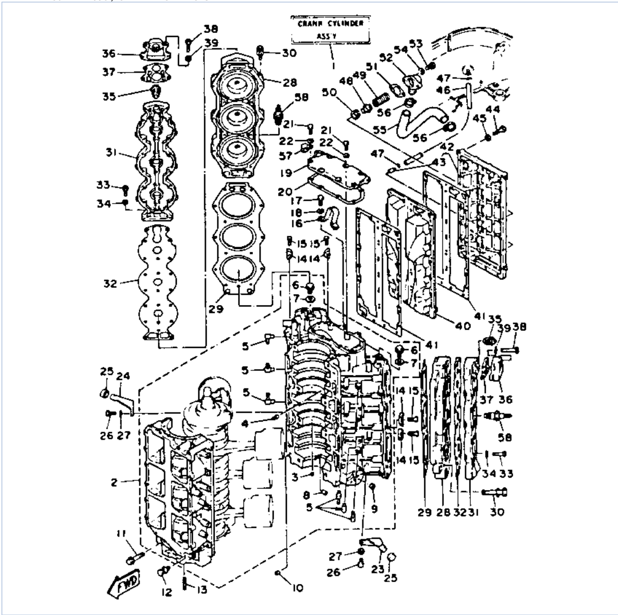
L150TXRR 1993 / CYLINDER CRANKCASE
