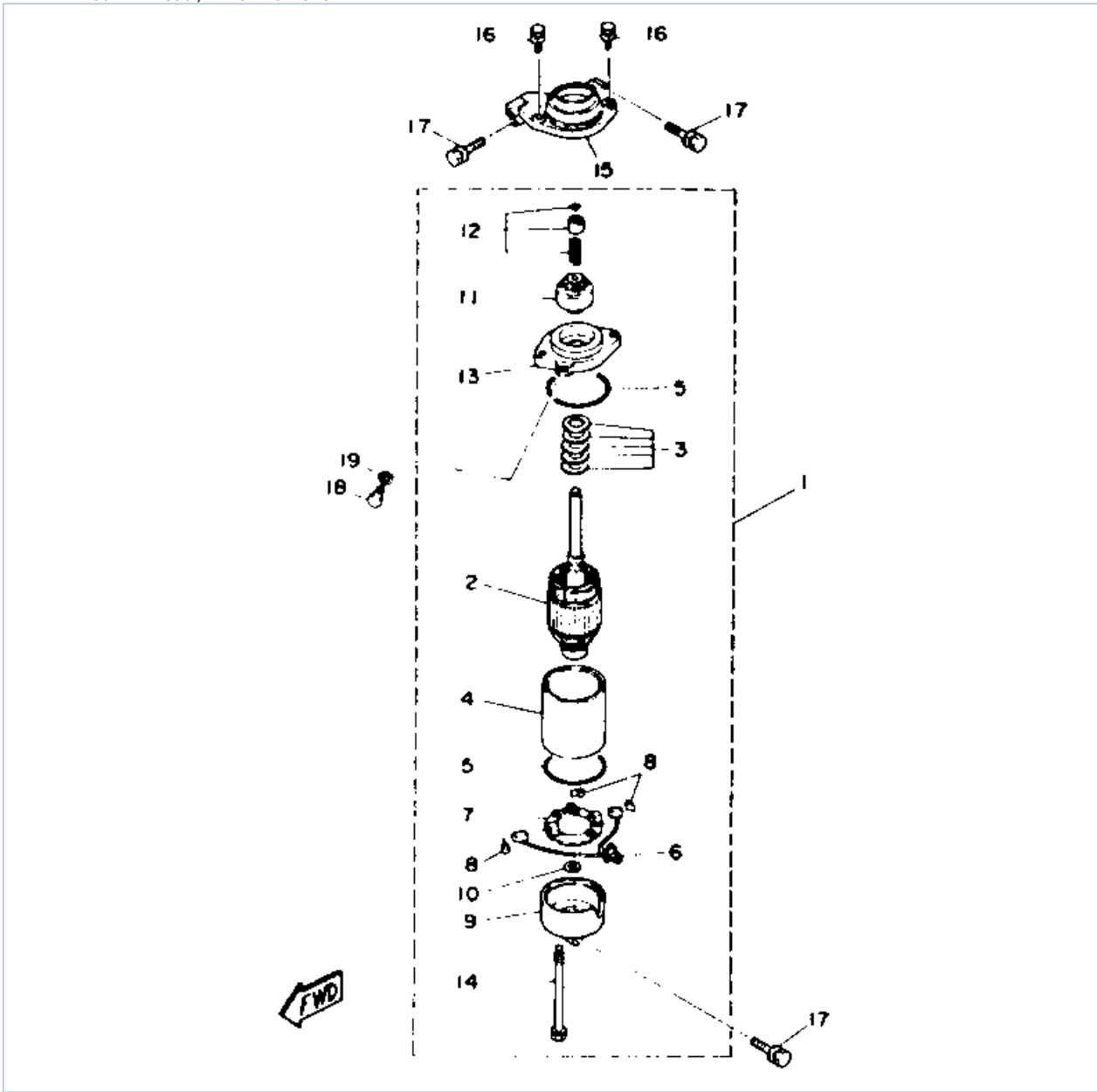
L150TXRR 1993 / ELECTRIC MOTOR
