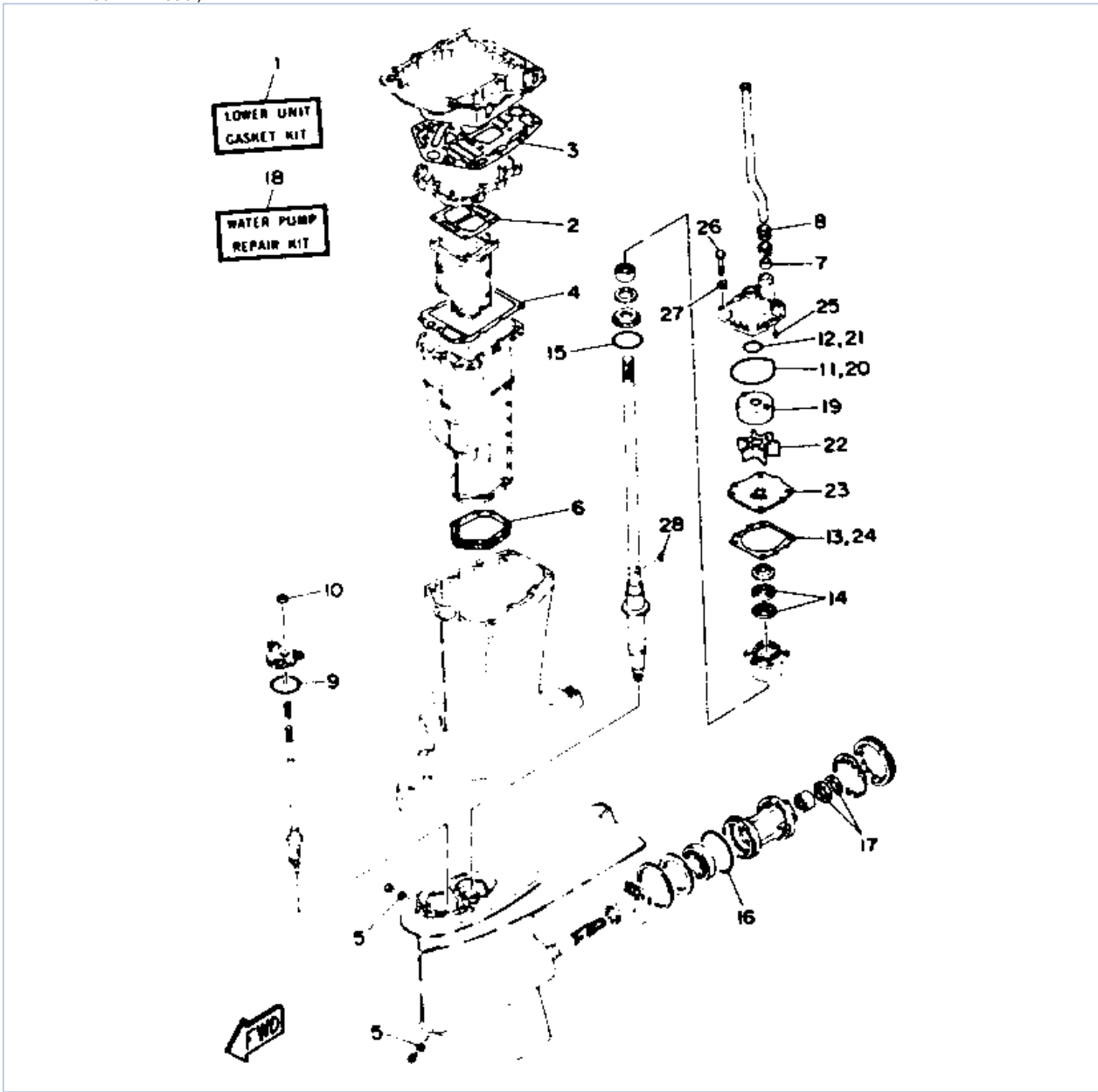
L150TXRR 1993 / REPAIR KIT 2
