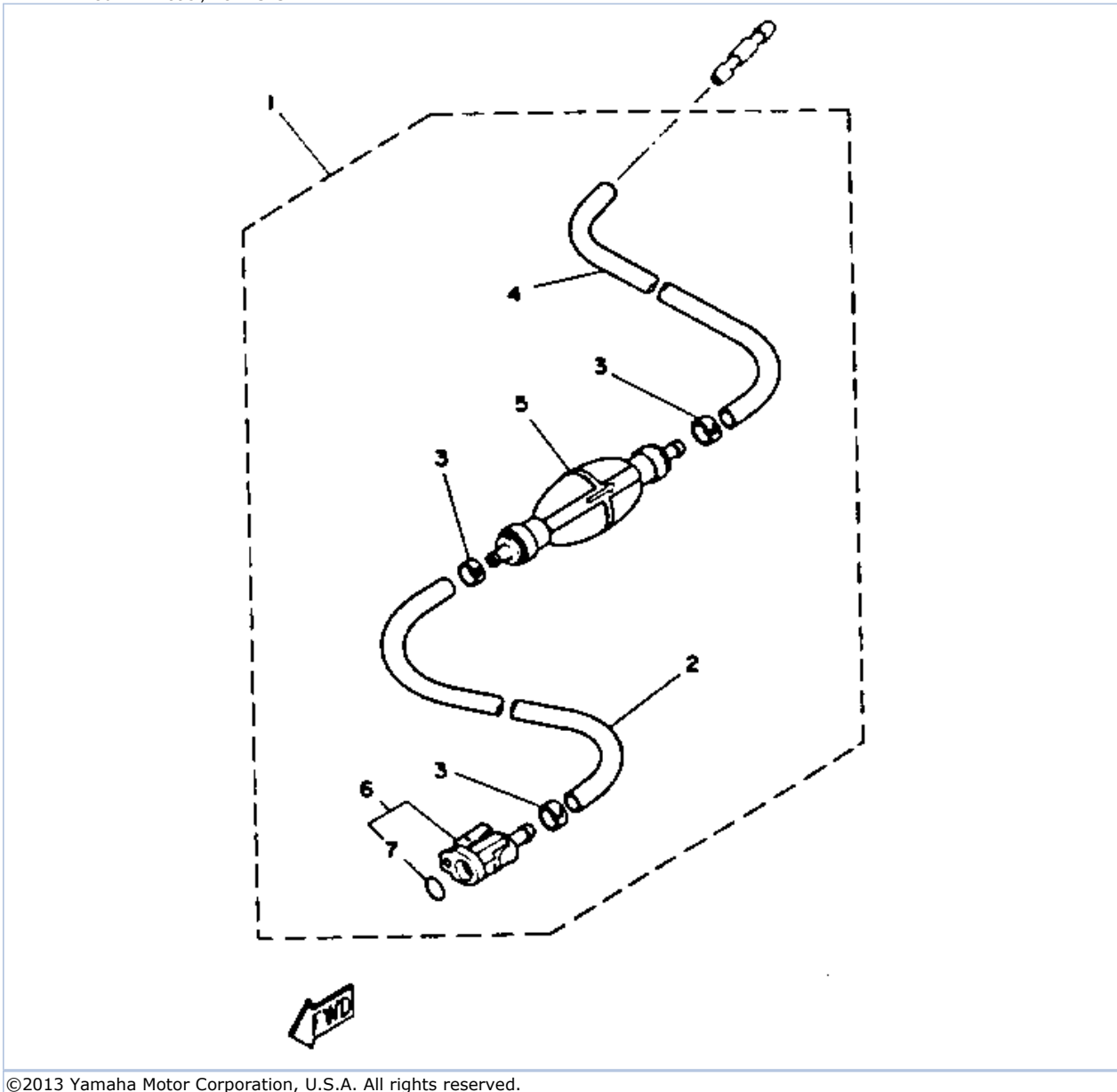
L150TXRR 1993 / FUEL SYSTEM 2
