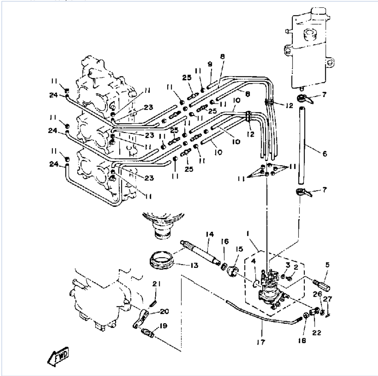
150ETXH 1987 / OIL PUMP
