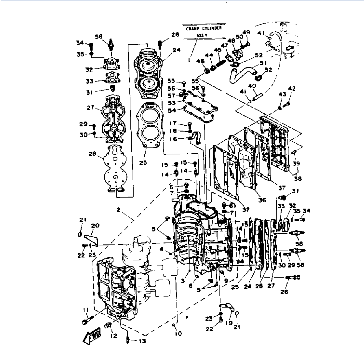
L130TXRP 1991 / CYLINDER CRANKCASE
