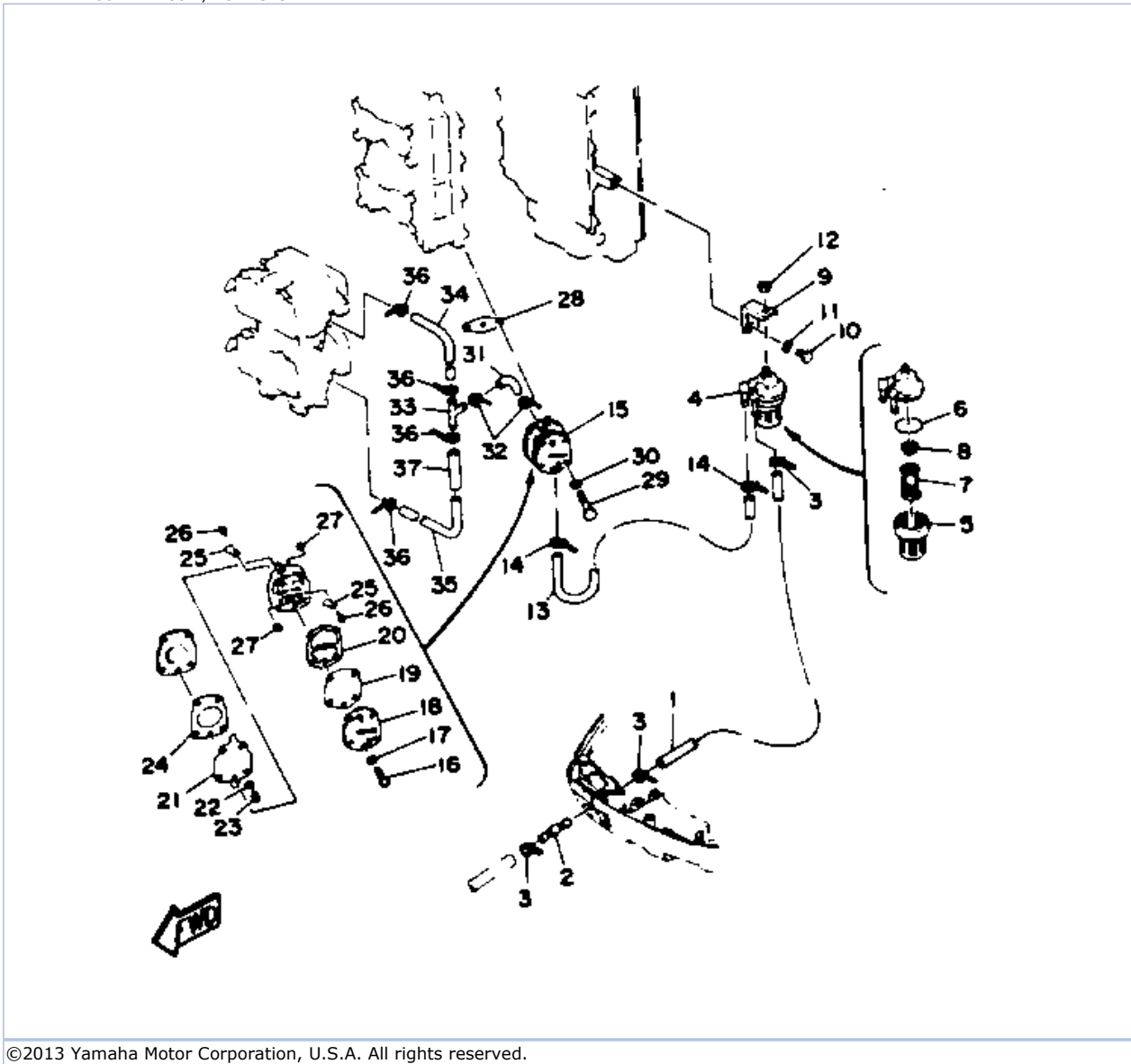
L130TXRP 1991 / FUEL SYSTEM 1
