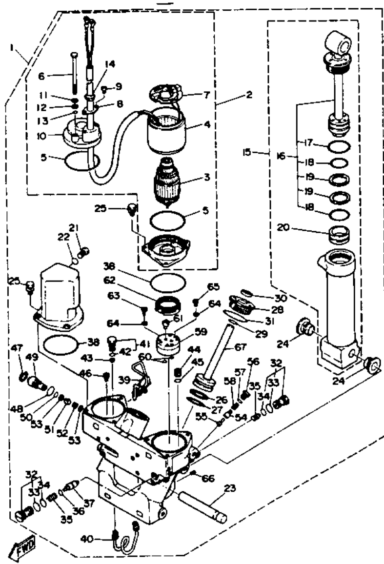
L130TXRP 1991 / POWER TRIM TILT ASSEMBLY 1
