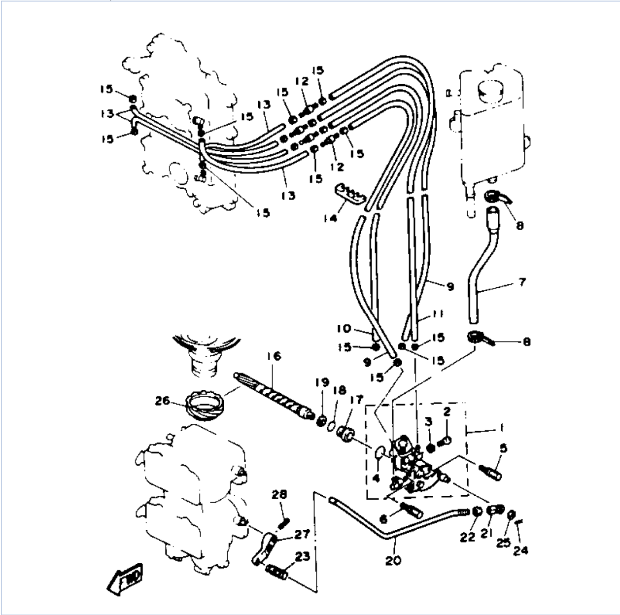
L130TXRP 1991 / OIL PUMP
