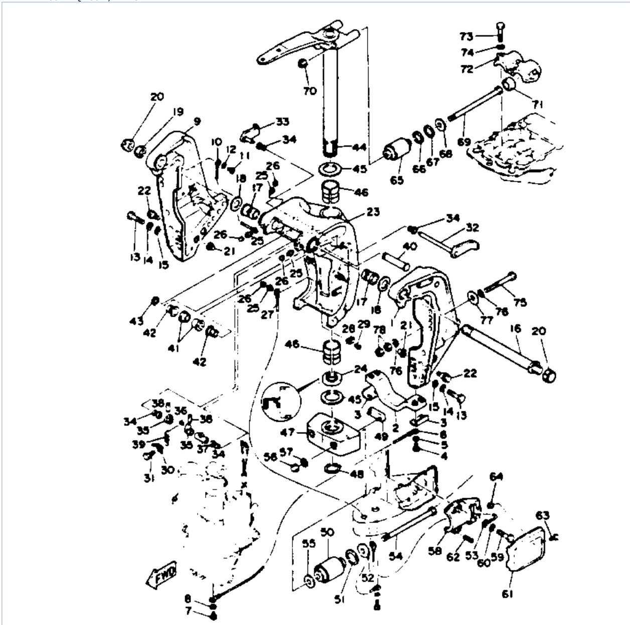
130TLRQ 1992 / BRACKET 1
