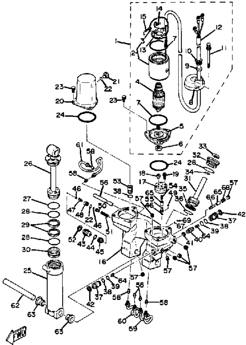
90ETLK 1985 / POWER TRIM TILT ASSY (- 453823)
