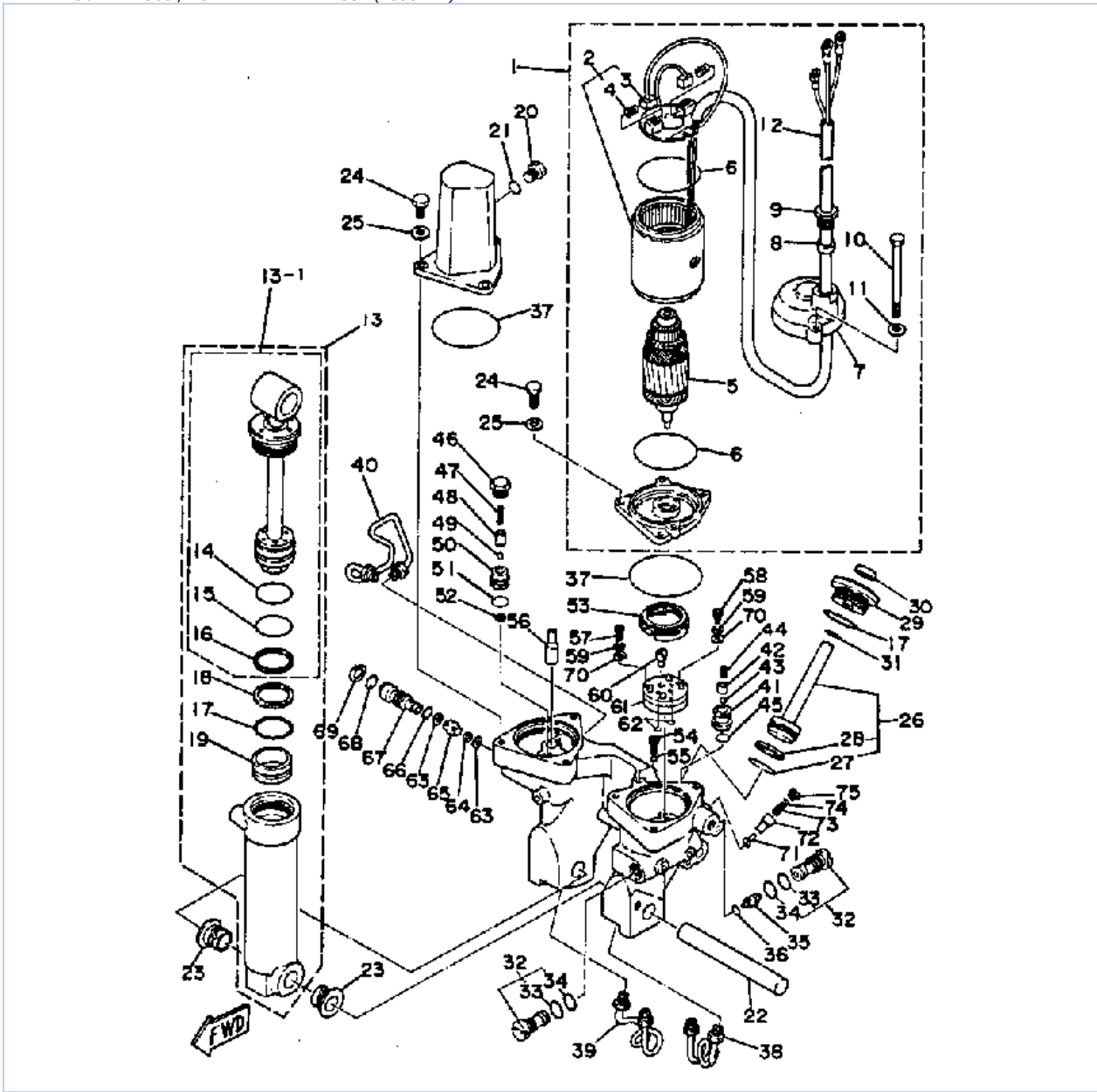
90ETLK 1985 / POWER TRIM TILT ASSY (453824 -)
