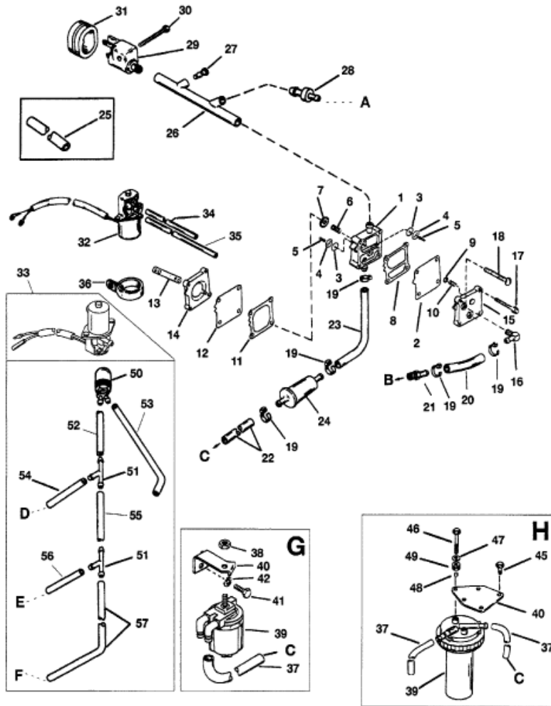
A = TO OIL PUMP, B = TO CRANKCASE, C = TO CARBURETOR, D = TO TOP CARBURETOR, E = TO CENTER CARBURETOR, F = TO BOTTOM CARBURETOR, G = DESIGN I, H = DESIGN II
