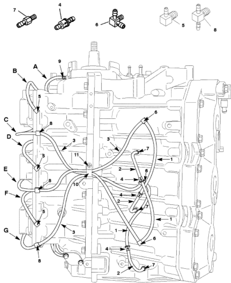
A THRU G = TUBING IS CONTINUED ON STARBOARD SIDE
