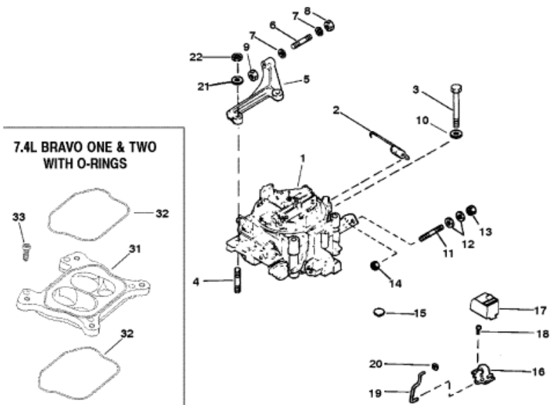
7.4L BRAVO ONE & TWO WITH O-RINGS
