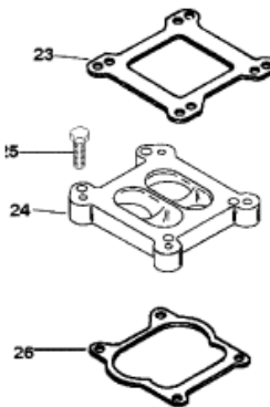
7.4L BRAVO ONE & TWO WITH GASKETS
